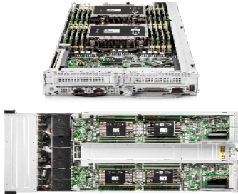
FIGURE 6. HPE Apollo 2000 Gen10 Plus system
